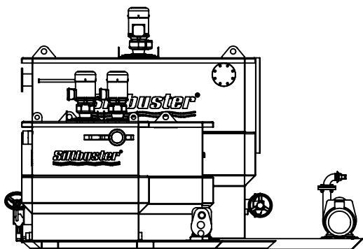
MT1 L: 2000mm W: 1200mm H: 1682mm H: 1205mm (BRIM) MT2 L: 2400mm W: 1600mm H: 1682mm H: 1205mm (BRIM) MT4 L: 3217mm W: 1400mm H: 2285mm H: 1810mm (BRIM)
