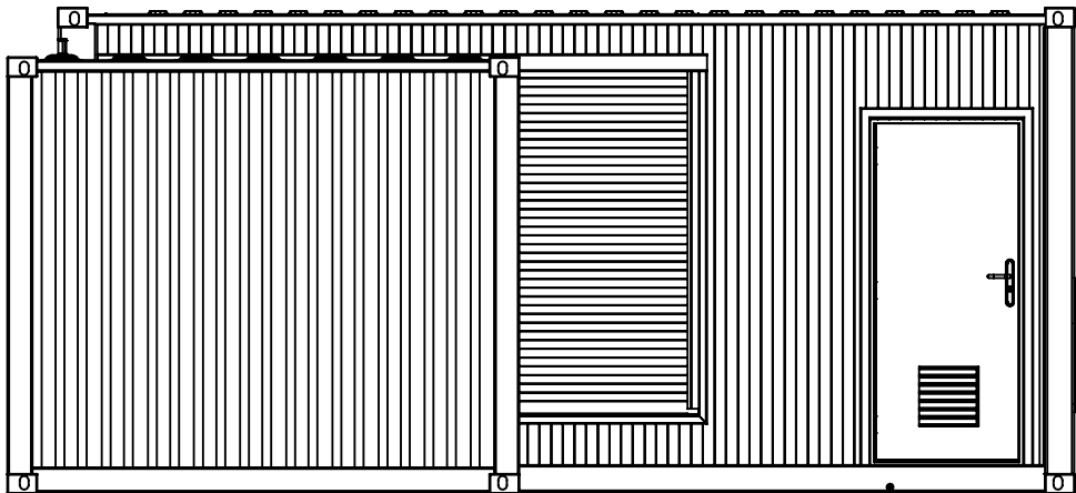
ISO10 DOSING CONTAINER L: 3050mm W: 2440mm H: 2600mm ISO20 DOSING CONTAINER L: 6060mm W: 2440mm H: 2890mm
