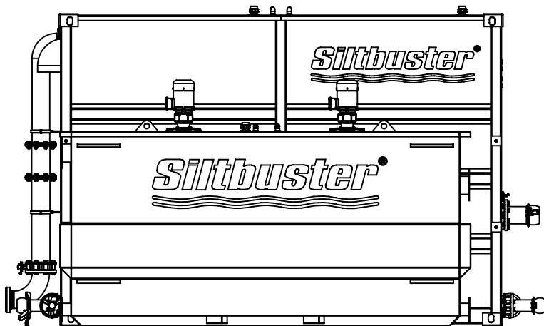
ISO10 DOSING CONTAINER L: 3050mm W: 2440mm H: 2600mm ISO20 DOSING CONTAINER L: 6060mm W: 2440mm H: 2890mm
